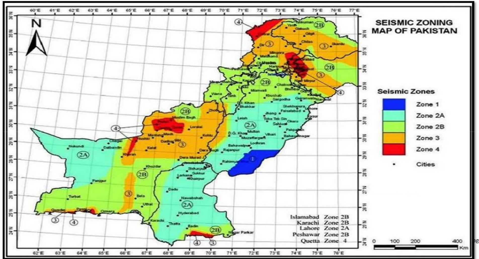
Figure 3: Seismic Zoning Map of Pakistan
